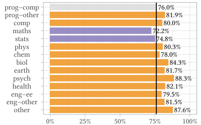
Figure 5: Weighted pass rates by category with all categories represented (the comparison line indicates the pass rate in prog-comp )
